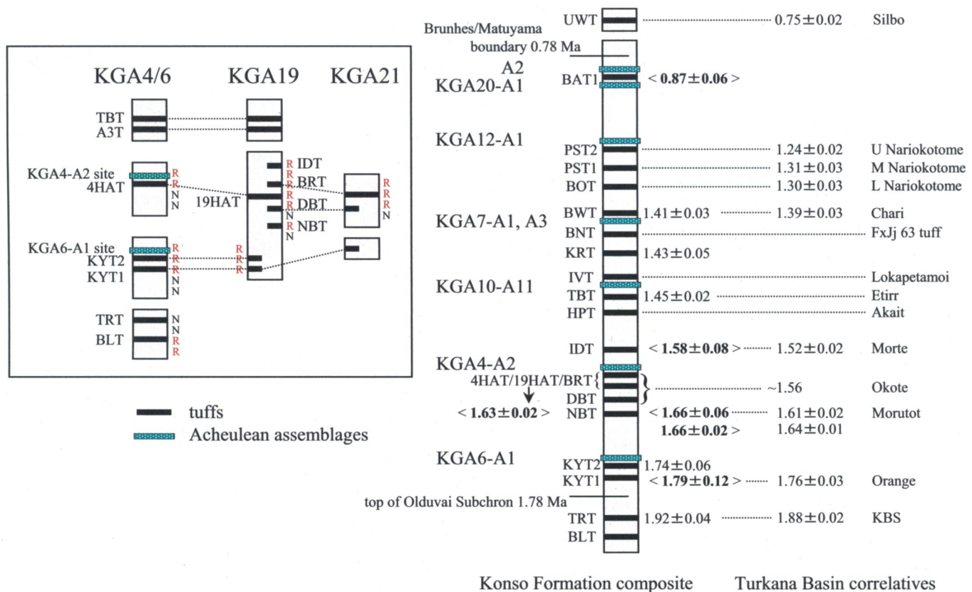
Fig. 1. Chronostratigraphic summary of the early Acheulean-bearing Konso Formation and correlation with the Turkana Basin tuffs. The geographic location of the Konso research area and locality positions are depicted in Suwa et al. (25). Dates in < > indicate new ^{40}\text{Ar}/^{39}\text{Ar} dates. Other dates are from Katoh et al. (20), McDougall and Brown (30), and McDougall et al. (31). All dates are weighted means adjusted to correspond to an FCs age of 28.2 Ma. Error margins are represented by population SDs. Left shows the schematic stratigraphy of the newly investigated KGA19 and -21 localities that enables a better chronological resolution of the Konso Formation time interval of ~1.45 to ~1.75 Ma. R and N indicate reverse and normal polarity intervals, respectively.
